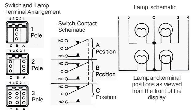
FIGURE IV- SCHEMATIC DIAGRAM
