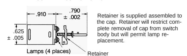
FIGURE III- PUSHBUTTON CAP WITH RETAINER
