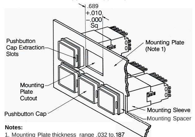
FIGURE II- MOUNTING
